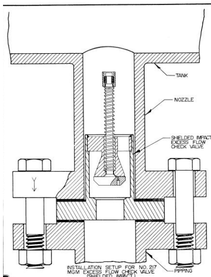
Figure 1: Installation Schematic
